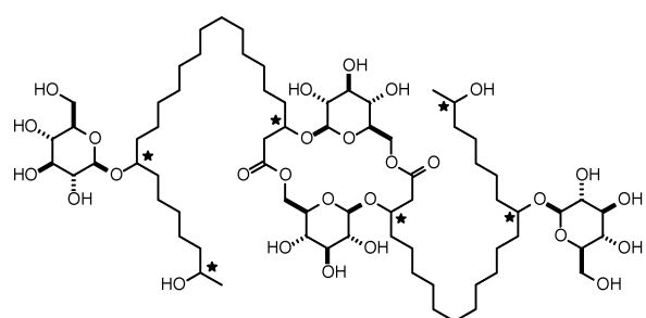
proposed structure of Fattiviracin FV-8 (2)
