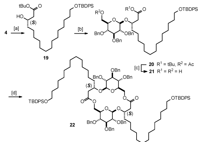
Scheme 6 a
