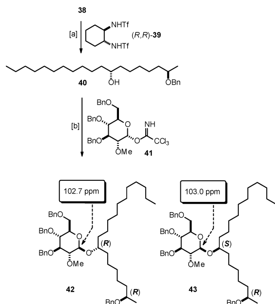
Scheme 10 a
