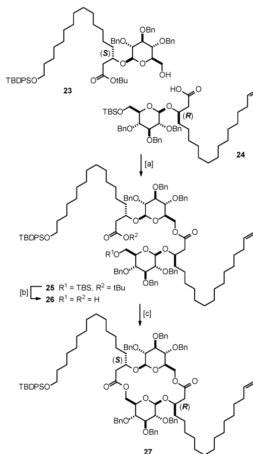
Scheme 7 a
