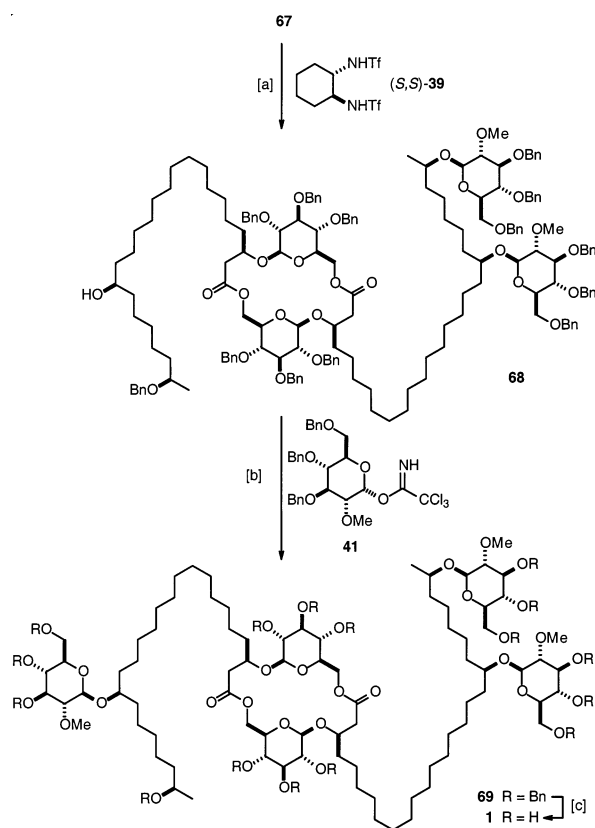
Scheme 15 a
