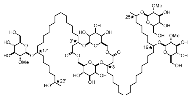
Cycloviracin B 1 (1)
