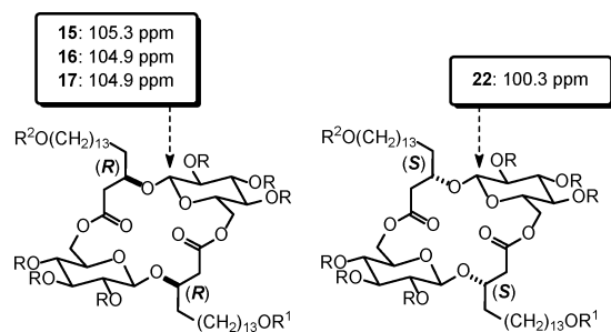
Scheme 5 a
