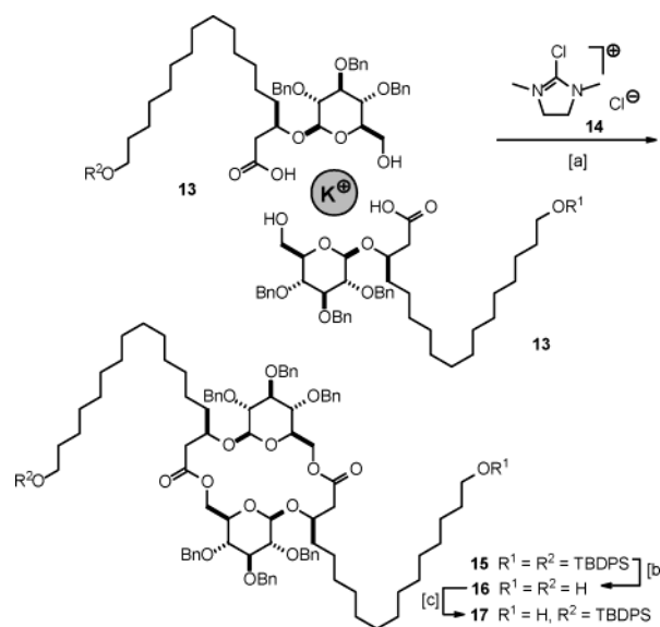
Scheme 4 a
